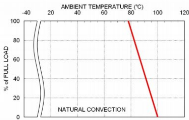
43RDL03-110S05W Derating Curve
