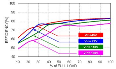
43RDL03-110S05W Efficiency vs. Output Load
