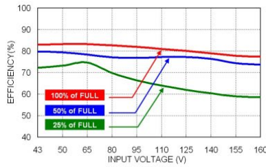
43RDL03-110S05W Efficiency vs. Input Voltage
